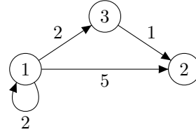
FIG. 1.3. Weighted system over \text{Trop}
