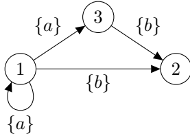
FIG. 1.2. Weighted system over \text{Lang}_A
